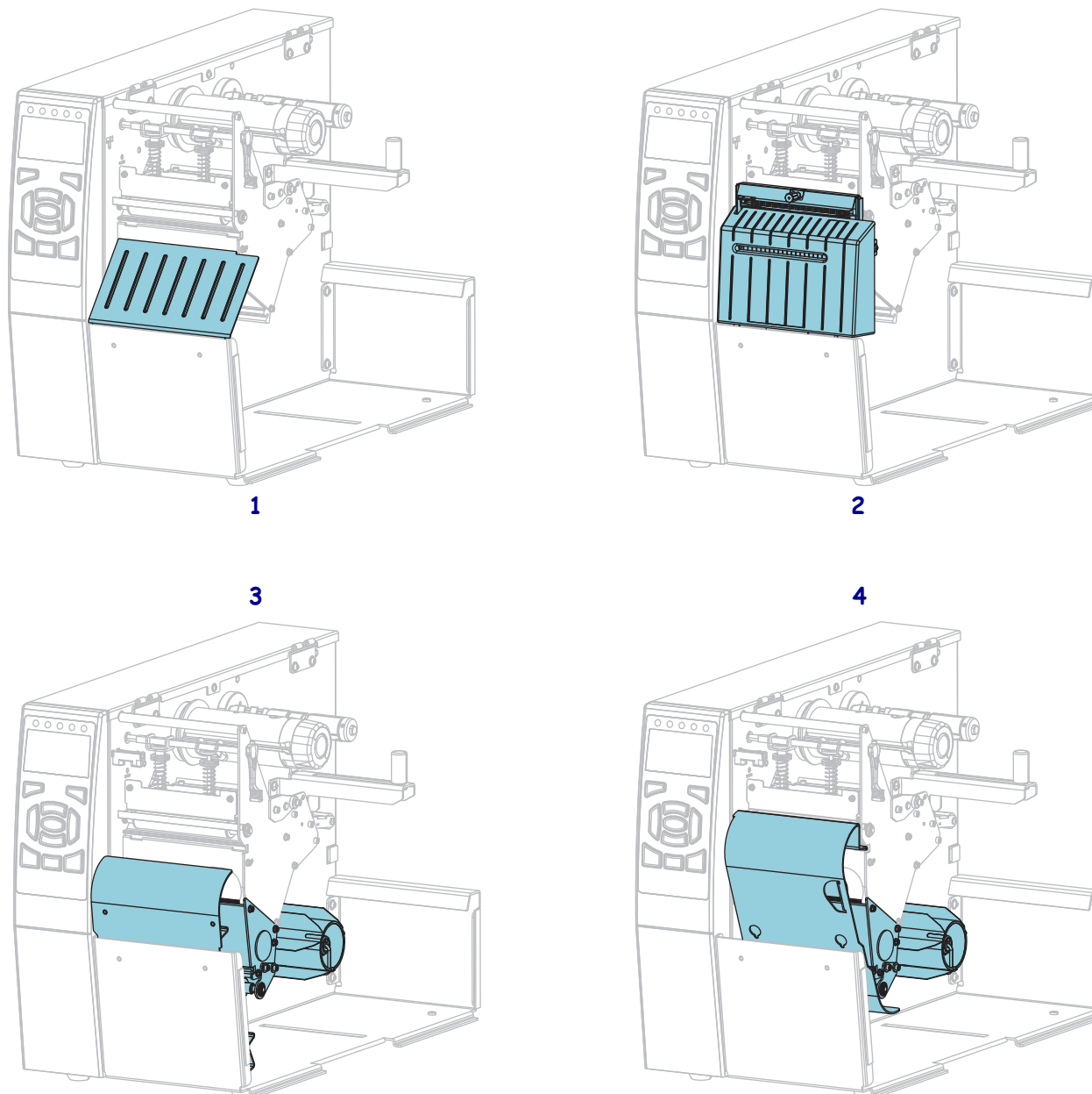
Figure 2 • Printer Options
