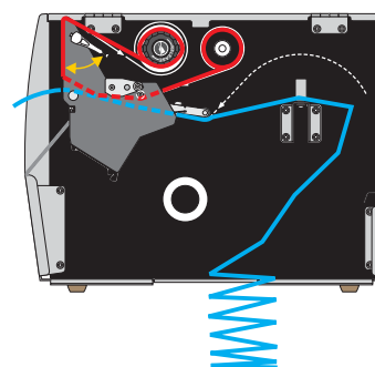
Bottom Feed
