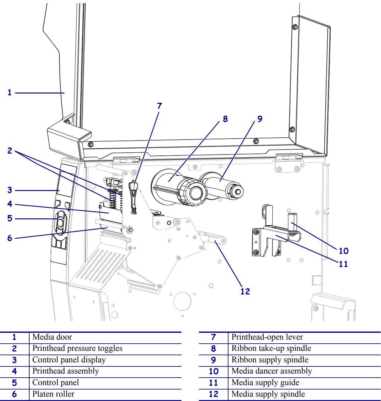
Figure 1 • Printer Components
