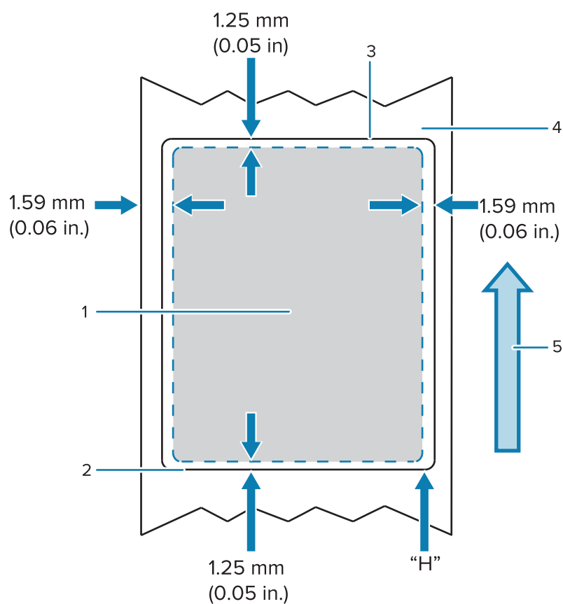
Figure 23 Gap Media
