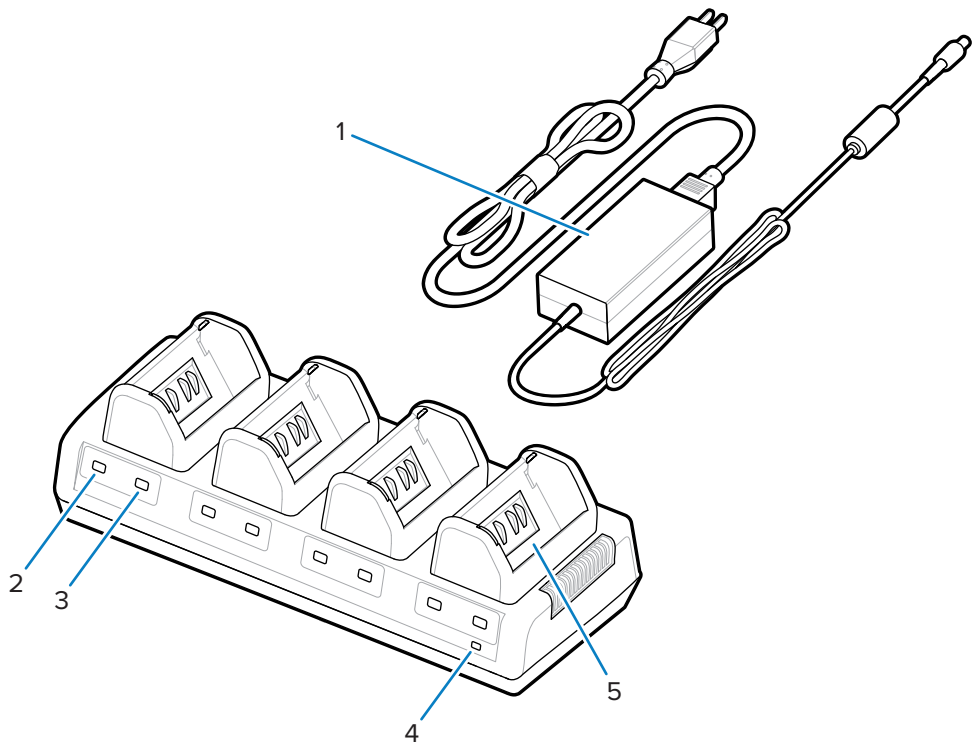
Figure 14 Quad Charger
