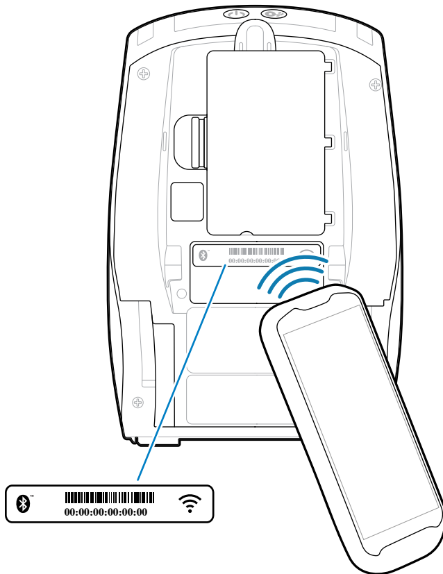
Figure 28 BT/WLAN Communications
