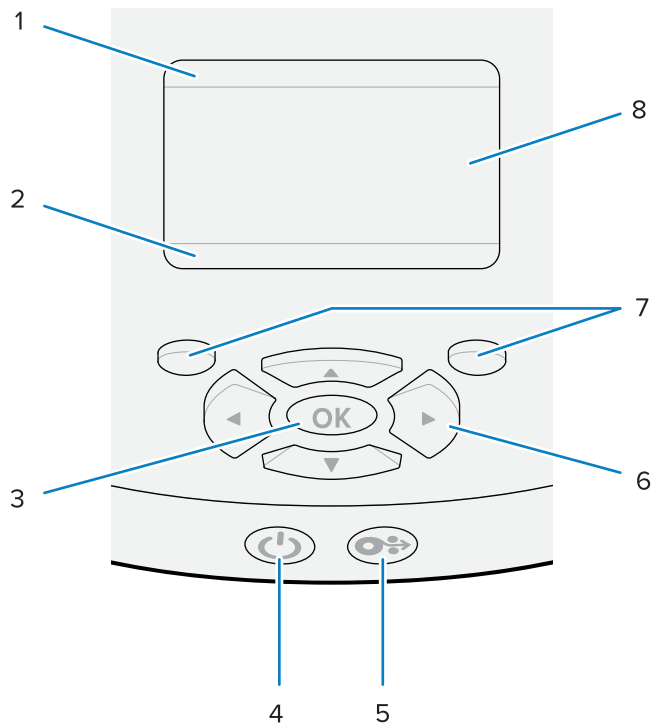
Figure 8 Control Panel
